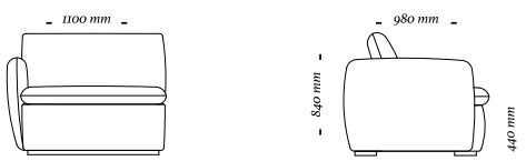
Mod 900mm c/ 1 br 1100x980x840mm
