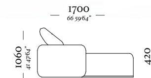
Chaise retratil Ass. 900mm C/ iBR S/ enfeite 1320x1200x860mm
