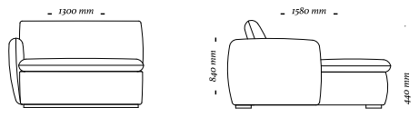
Chaise Longue 100mm c/ 1 br 1300x1580x840mm
