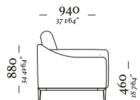
Poltrona Ass. 700mm C/ 2BR 1210x940x880mm
