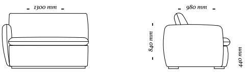
Mod 100mm c/ 1 br 1300x980x840mm
