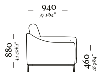
Poltrona Ass. 900mm C/ 2BR 1400x940x880mm
